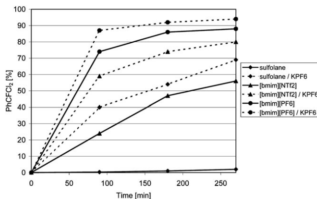
Figure 4. Activation of fluorination by KPF 6 in ionic liquids and sulfolane (GC analysis).
