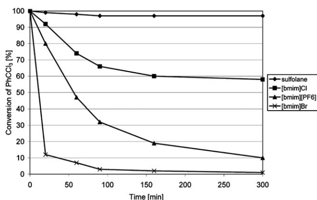
Figure 1. Fluorination in three ionic liquids and sulfolane (conversion of 1 , GC analysis).
