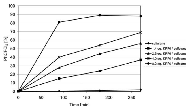
Figure 5. Effect of the amount of KPF 6 on the fluorination by KF in sulfolane (GC analysis).
