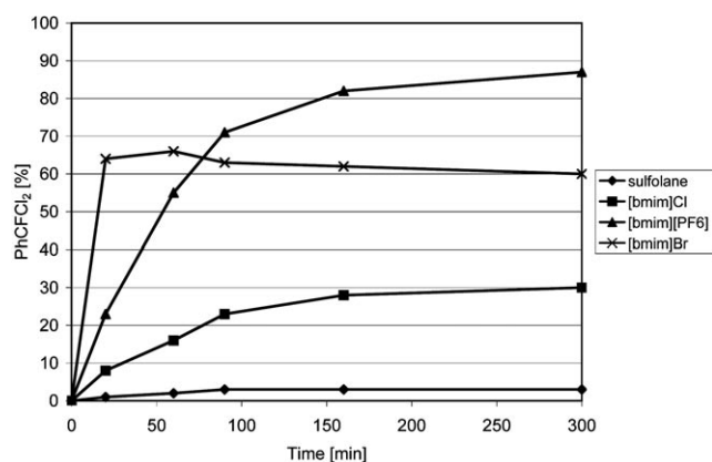
Figure 2. Fluorination in three ionic liquids and sulfolane (formation of 2 , GC analysis).
