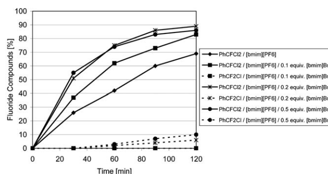
Figure 3. Activation of the fluorination by using various amounts of [bmim]Br (GC analysis).
