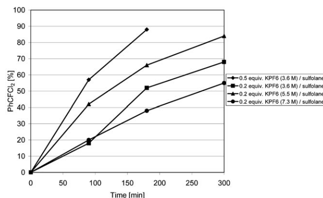
Figure 6. Effect of the concentration of KPF 6 in sulfolane, on the fluorination by KF (GC analysis).
