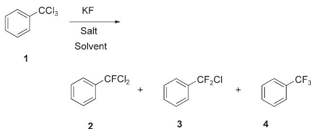
Scheme 1. Fluorination of trichlorotoluene.
