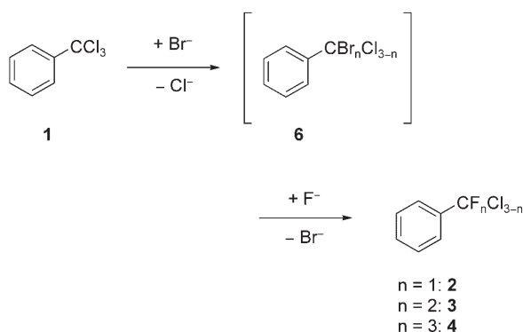
Scheme 2. Activation by \text{Br}^- during the fluorination of trichlorotoluene.
